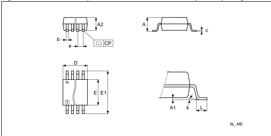
Figure 13. SO8W – 8 lead plastic small outline, 208 mils body width, package outline
